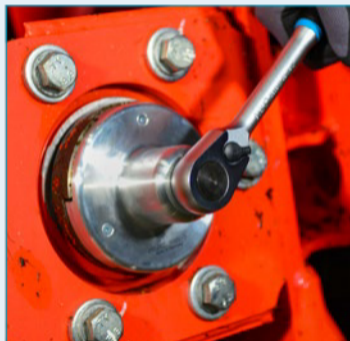
Operating using ratchet with inserted 12.5 mm (1/2") 4-point socket
