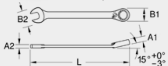
BT013806... 832 Ratchet ring spanner, reversing
