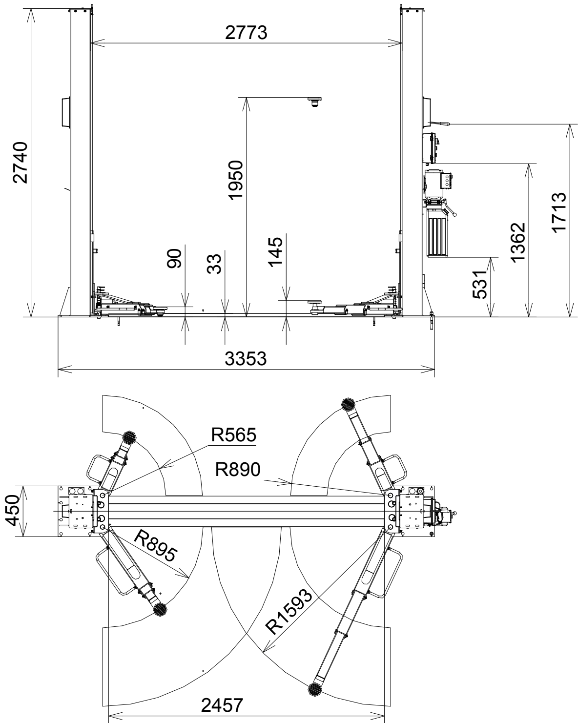
Figure 3 – LAYOUT
